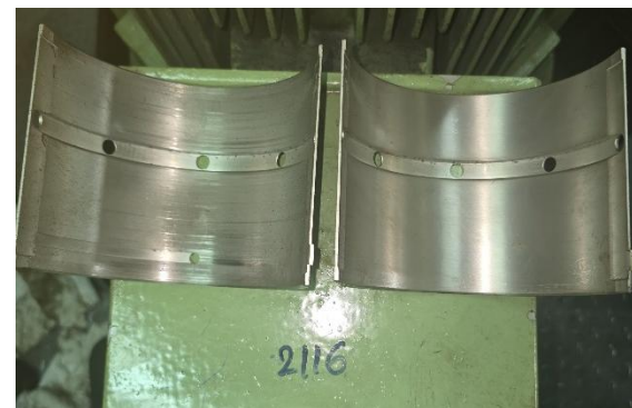
WHEEL GEAR ROTOR BEARING SHELLS & THRUST BEARING METALS
