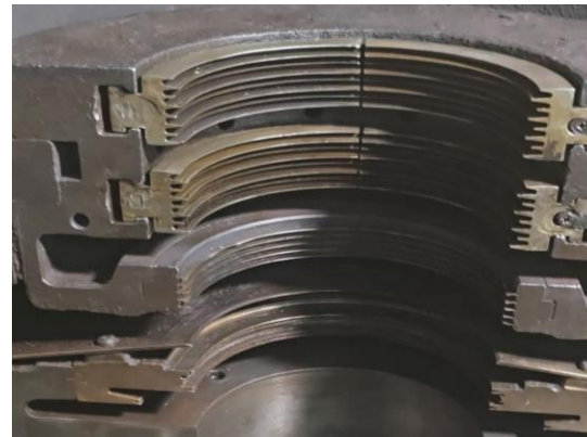
LABYRINTH PACKING (8 SEGMENTS), STEAM GUARD (1 PAIR) & OIL GUARD (1 PAIR) AFTER CLEANING
